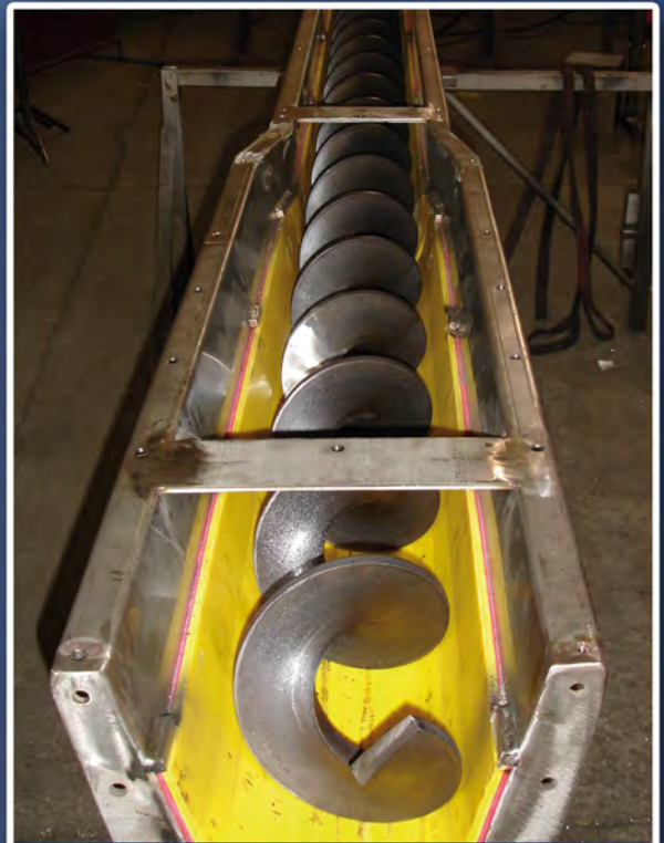
"ATEX" CONVEYOR FOR SLURRY
